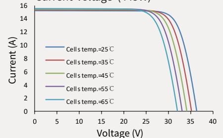
Current-Voltage (445W)
